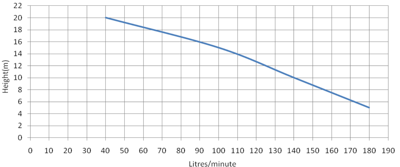
Pump Performance
